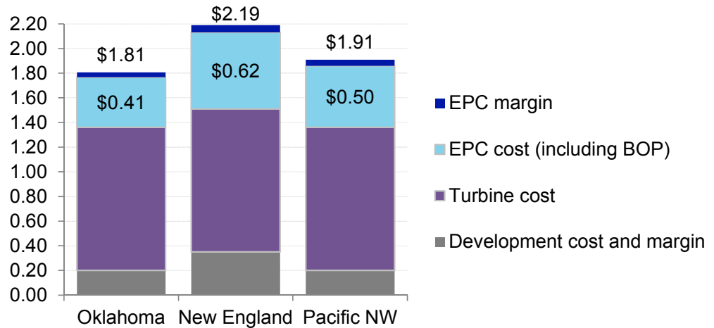
Figure 3: Wind – estimated EPC costs and overall project economics for a 50MW project across various US regions ($/W DC )
