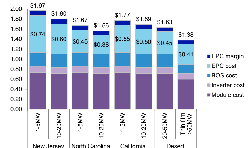
Figure 2: Solar – estimated EPC costs and overall project economics for different project sizes across various US regions (excludes developer costs and margins) ($/W DC )
